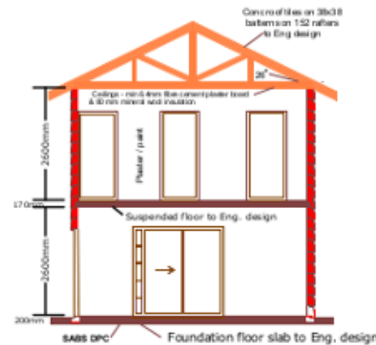
Section XX
